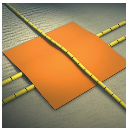
Illustration of a Njord Polymat in position at a pipeline/cable crossing
