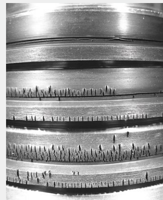
Competitor products strained at 10%, 20%, 30%, and 40% failed after 24 hours at all four strain levels with ozone exposure.
