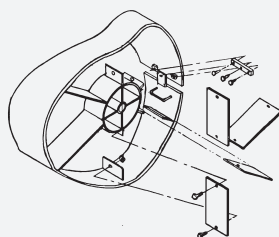
Exploded View
