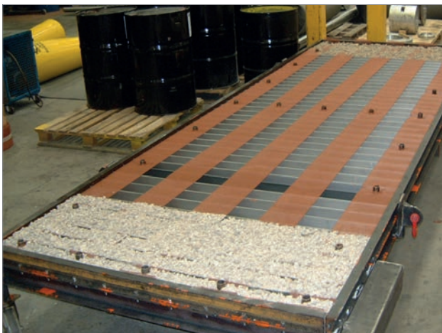
Ballast and reinforcement inside the Polymat™
