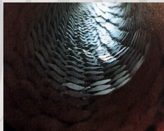
Hose inside after 28 months of use
