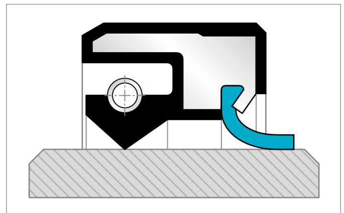
Figure 7: Elastomer/Turcon® Hybrid. This combination utilizes the best attributes of both a Radial Oil Seal and Turcon® Varilip® PDR.
