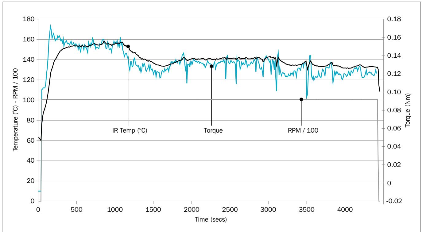
Figure 10: Running torque for Turcon® Varilip® PDR
