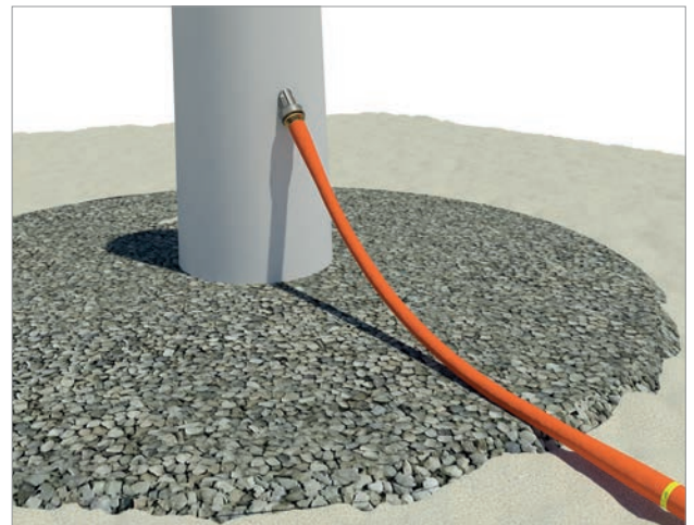
Schematic of NjordGuard™ installation in the monopile
